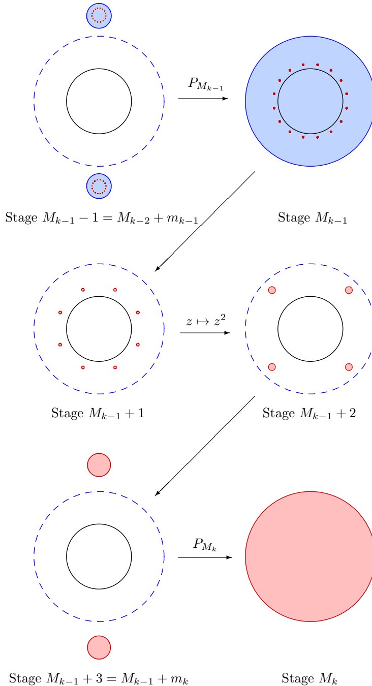
FIGURE 1. How the survival sets \mathcal{S}_k are nested. The pictures show preimages of \overline{D}(0, 2) at stages M_k (in red) and M_{k-1} (in blue) with m_k = 3 . The dashed blue circle is C(0, 2) while the unit circle is shown in black. Observe how Q_{M_{k-1}, M_k}^{-1}(\overline{D}(0, 2)) \subset \overline{D}(0, 2) \setminus \overline{D}(0, 1) as in Remark 1(c) is shown in red in Stage M_{k-1} .
