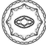
FIGURE 1. The Julia set of G = \langle h_1, h_2 \rangle , where we set g_1(z) := z^2 - 1, g_2(z) := z^2/4, h_1 := g_1^2, h_2 := g_2^2 . G \in \mathcal{G}_{dis} and G is hyperbolic.
